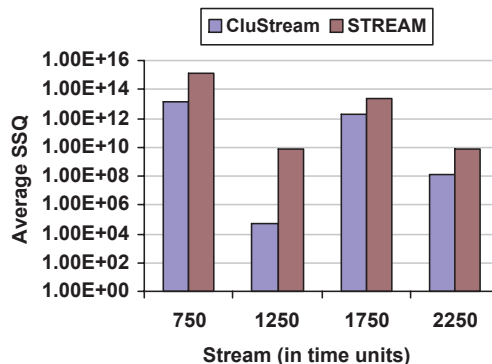
Figure 2: Quality comparison (Network Intrusion dataset, horizon=256, stream_speed=200)
