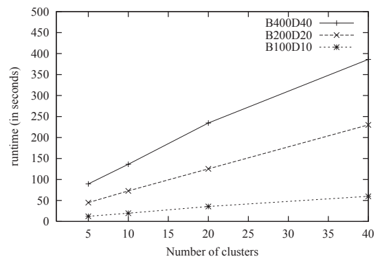
Figure 8: Scalability with Number of Clusters (stream_speed=2000)
