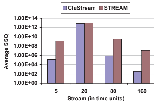
Figure 1: Quality comparison (Network Intrusion dataset, horizon=1, stream_speed=2000)
